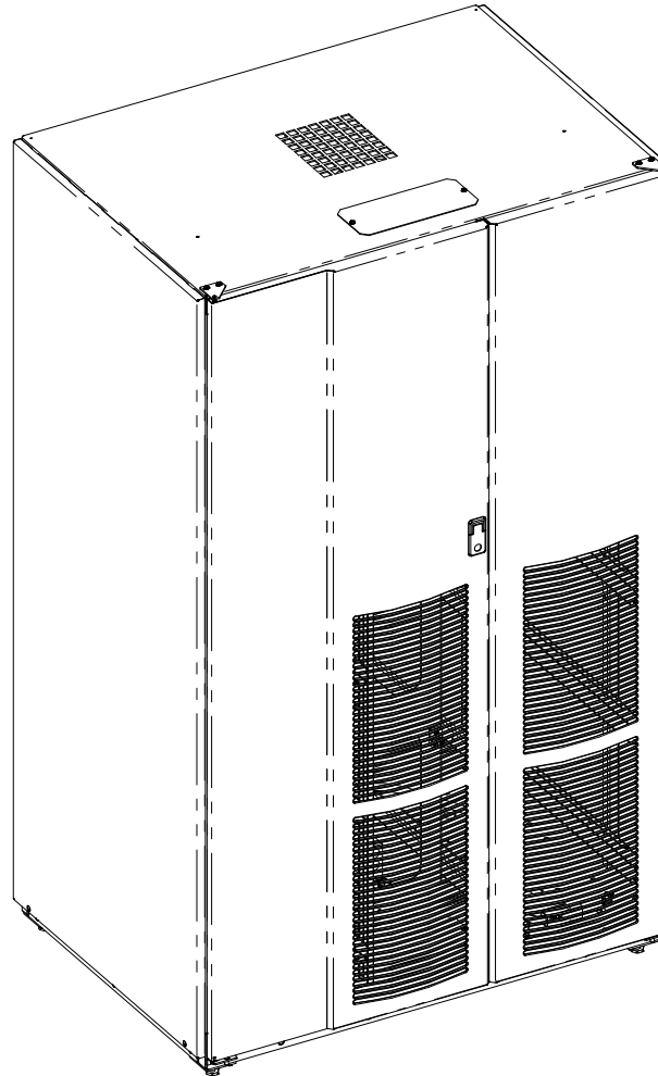
Figure 1-1. Typical Eaton 9395 Model 1085 or 1085HR Battery Cabinet
