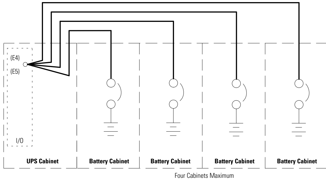
Figure 5-1. Battery Cabinet Online – Common Battery (275 and 500 kVA RT and 275 kVA Plus 1 UPS)
