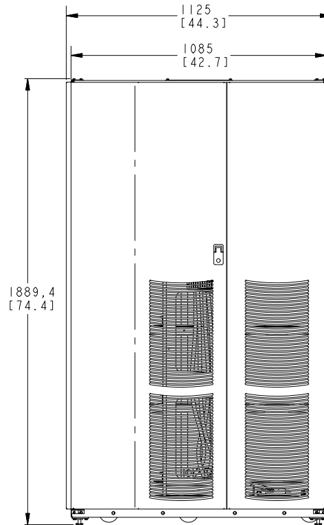
Figure 3-1. Model 1085 or 1085HR Battery Cabinet Dimensions (Front View)
