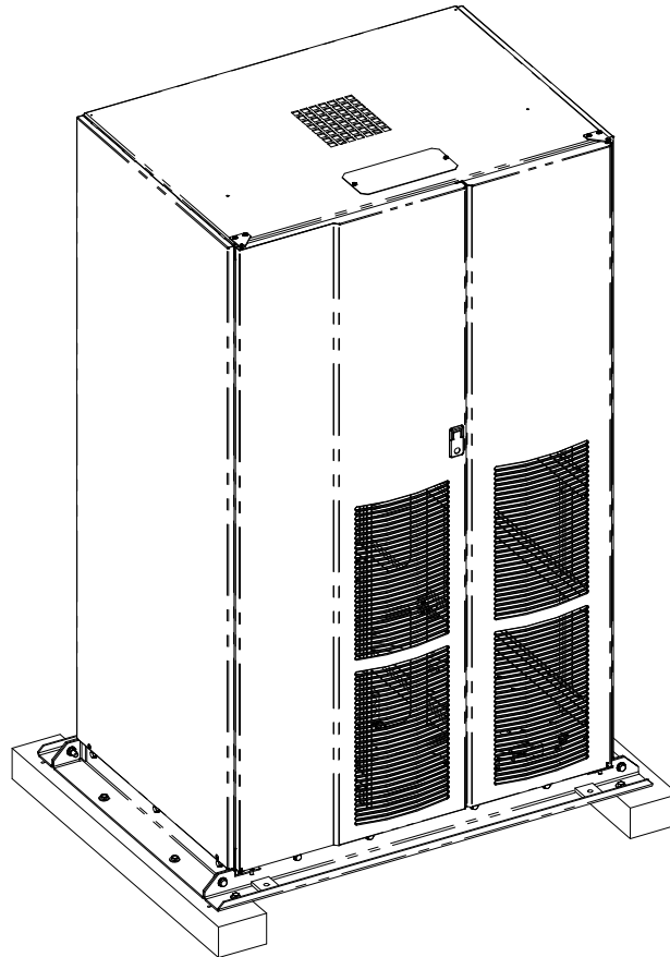
Figure 3-5. Eaton 9395 Model 1085 or 1085HR Battery Cabinet as Shipped on Pallet
