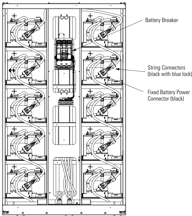
Figure 4-14. 1085HR Battery String Connection
