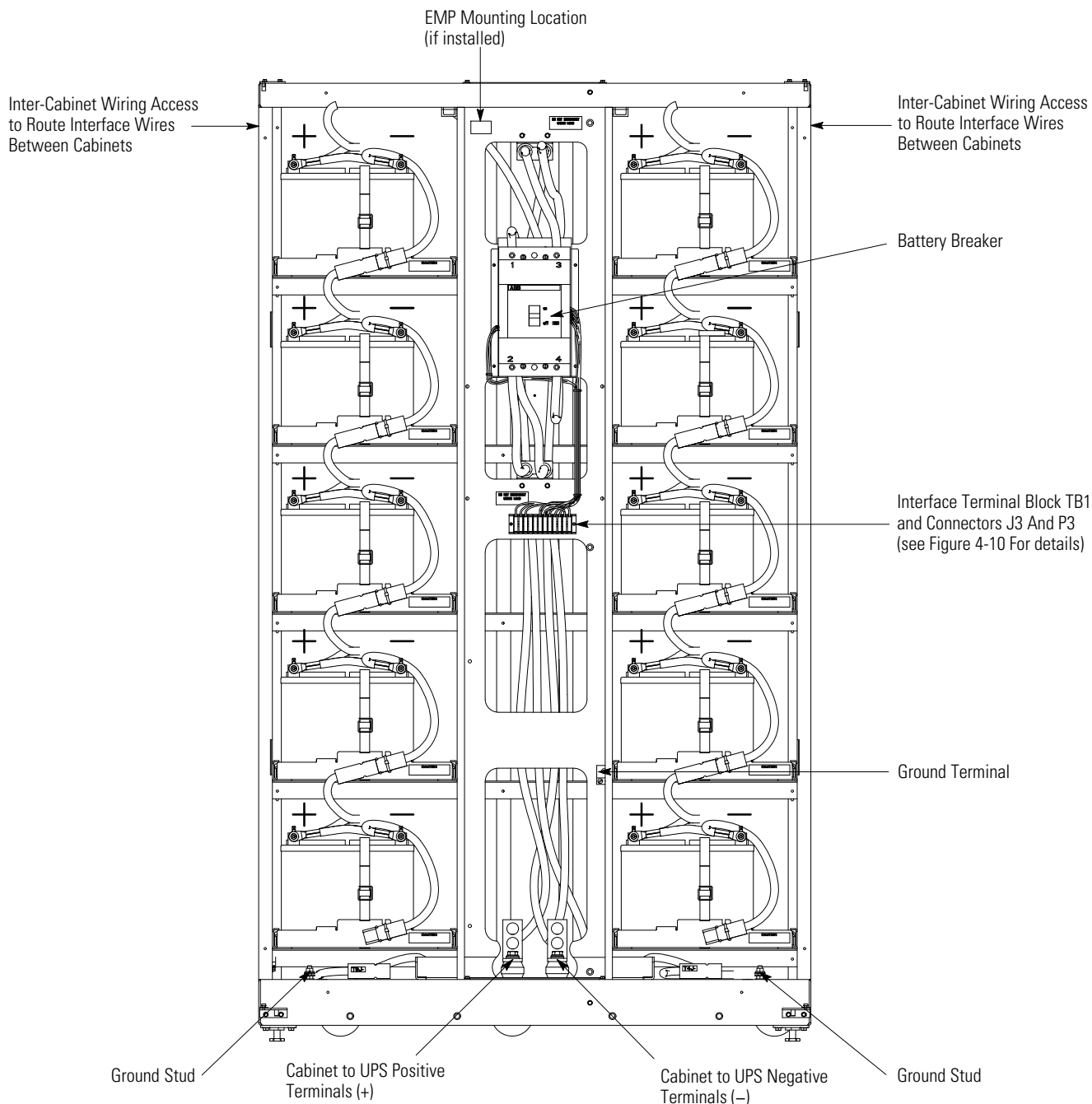
Figure 4-7. 1085 Battery Power and Interface Terminal Locations
