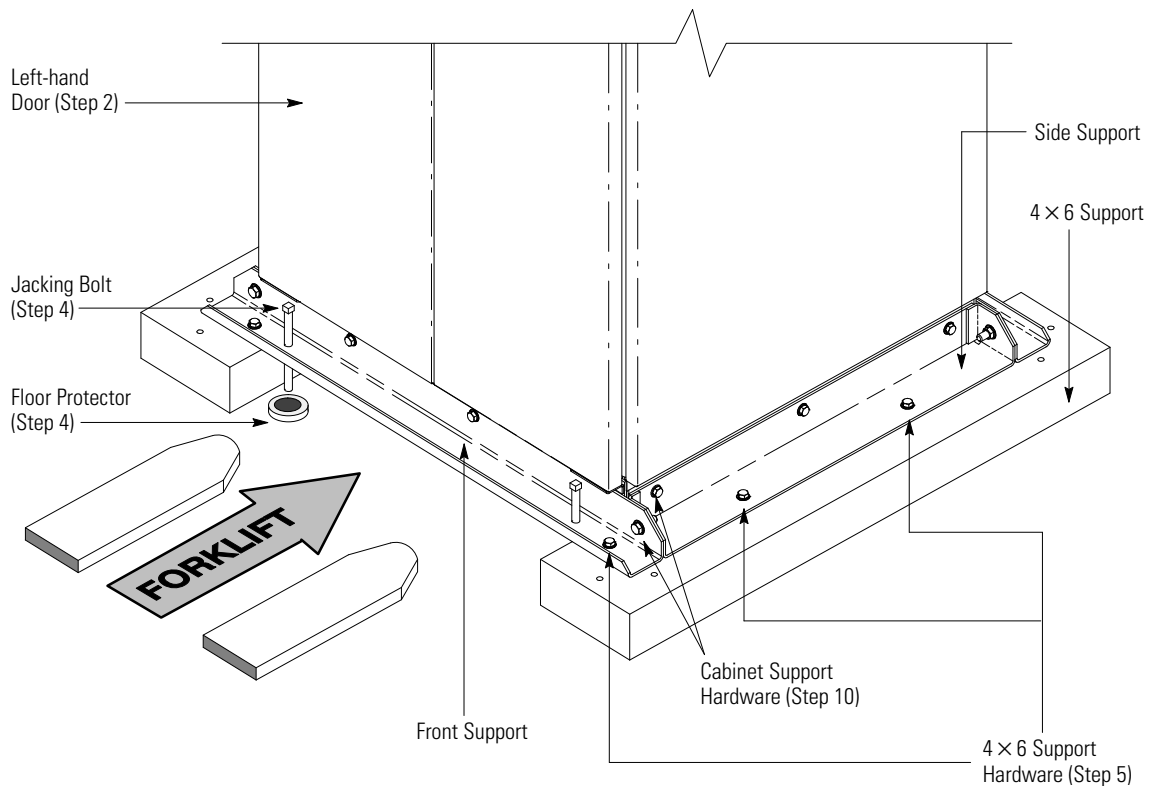
Figure 4-1. Removing Shipping Supports
