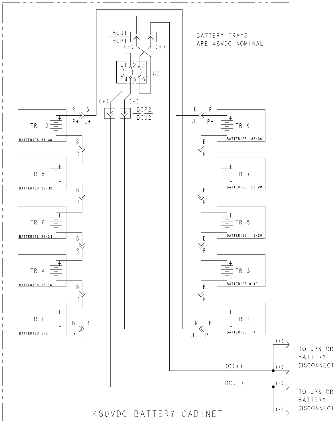
Figure 5-5. 1085 or 1085HR Battery Cabinet with Three-Pole Breaker Power Wiring Schematic
