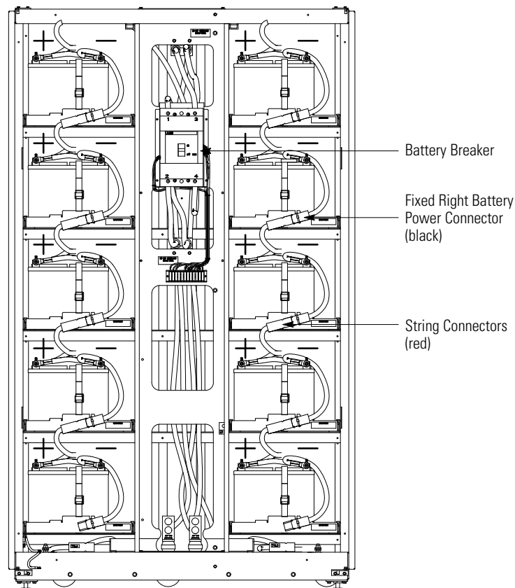
Figure 4-13. 1085 Battery String Connection
