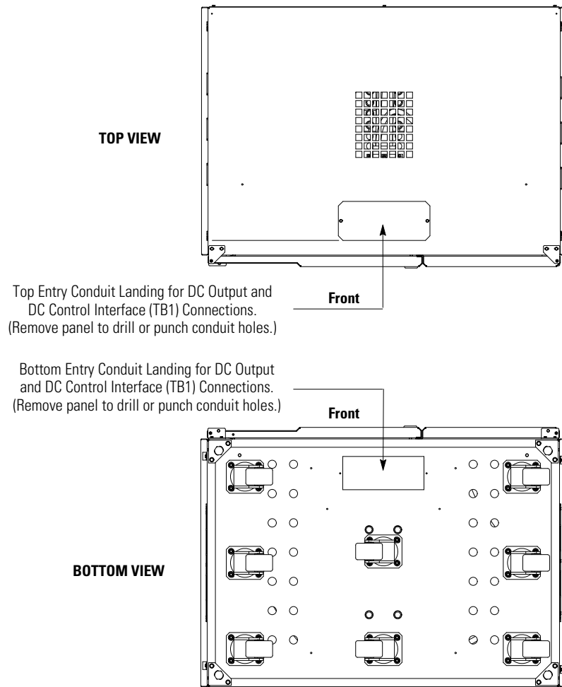
Figure 4-6. Battery Cabinet Conduit and Wire Entry Locations
