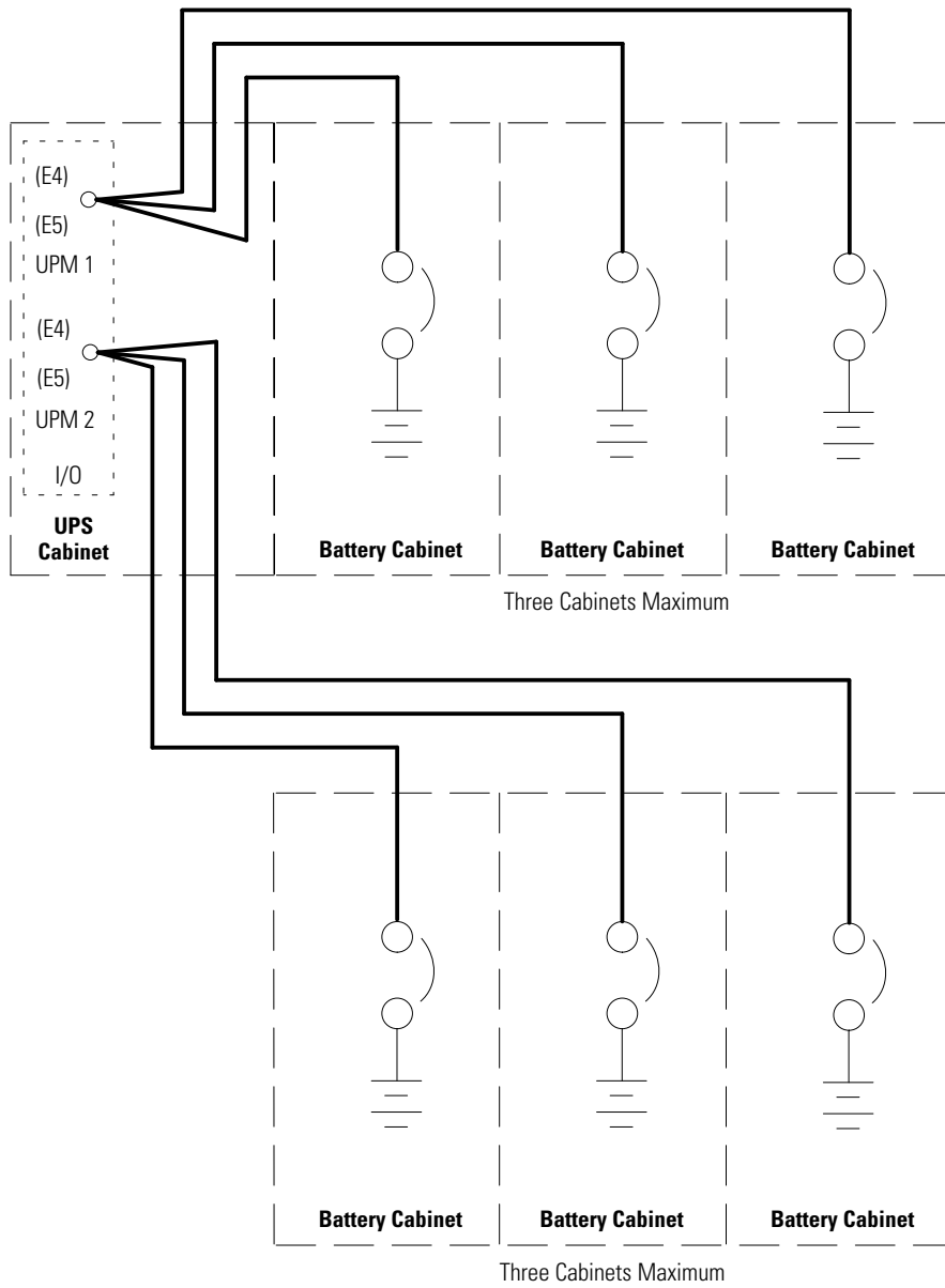
Figure 5-3. Battery Cabinet Oneline – Separate Battery (275 kVA Plus 1 and 500 kVA RT UPS)
