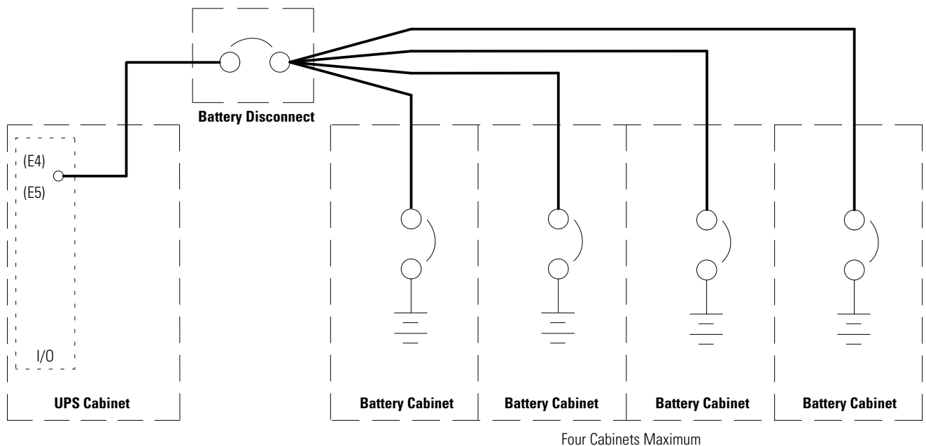
Figure 5-2. Battery Cabinet Online with Disconnect – Common Battery (275 and 500 kVA RT and 275 kVA Plus 1 UPS)
