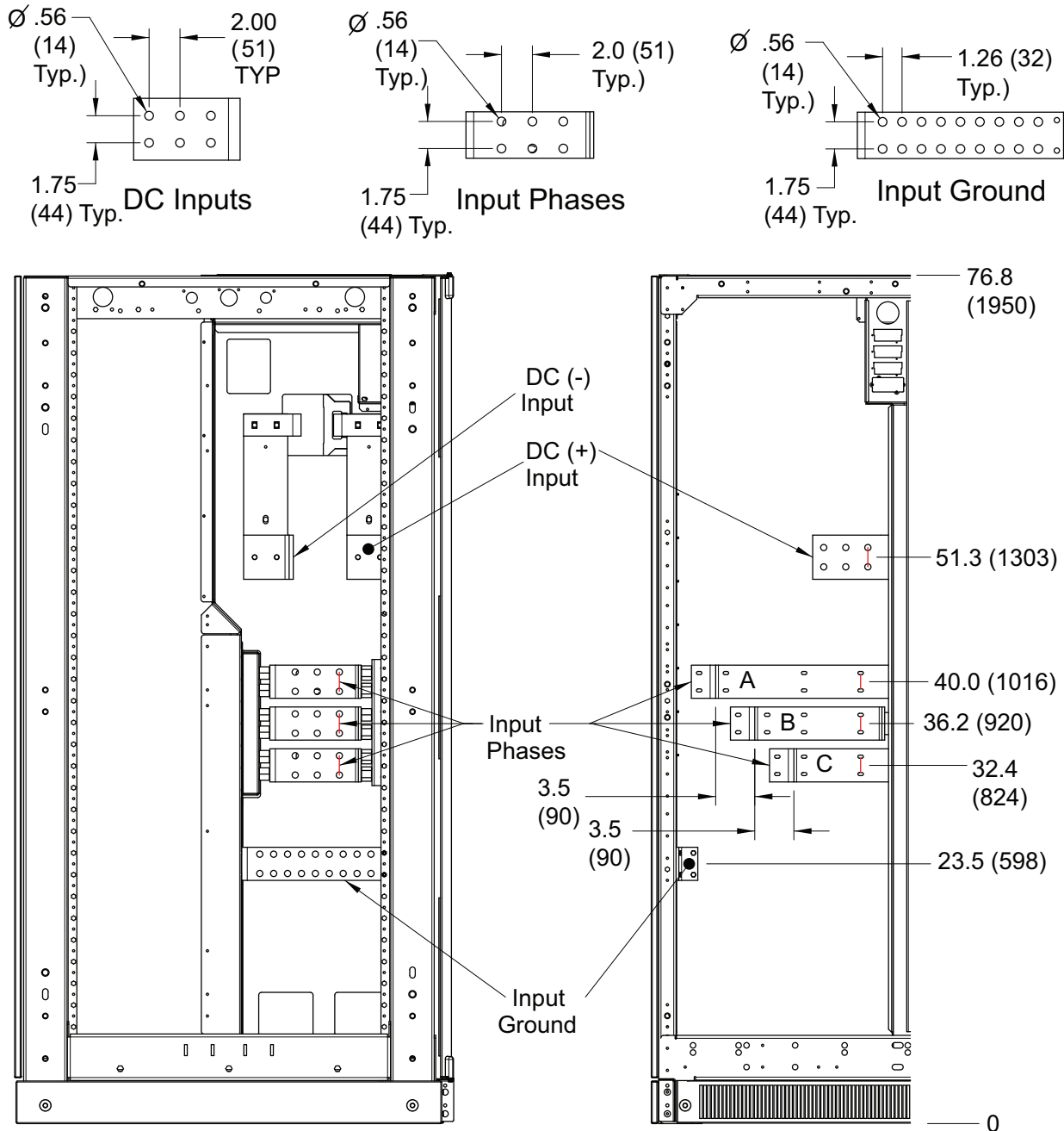
Figure 27 Input terminal detail, 625/750kVA Liebert NXL, N+1 multi-module unit without static bypass
