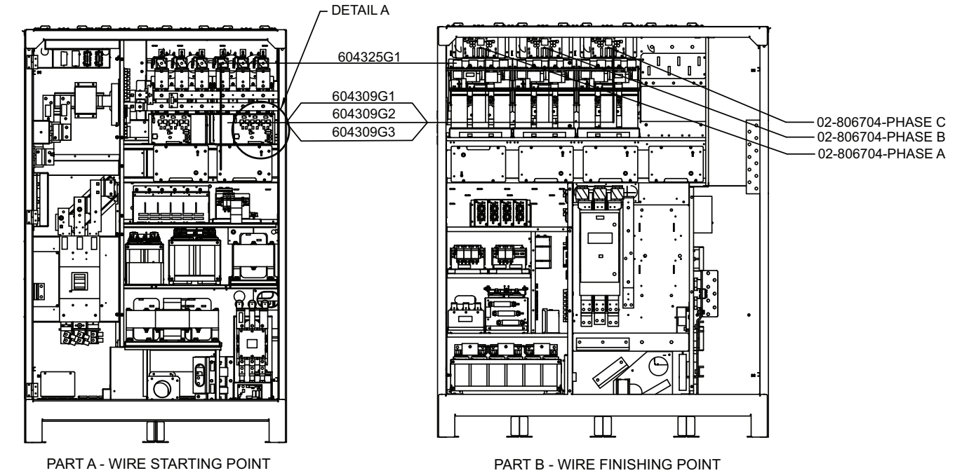
Figure 19 Field connections, shipping split 500kVA Liebert NXL, multi-module or SMS with static bypass, Page 1
