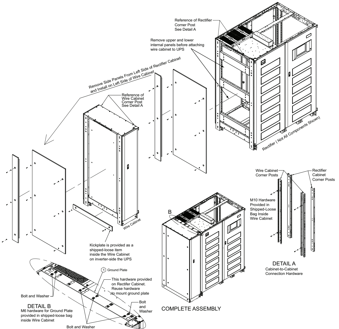
Figure 35 Single-input wire cabinet
