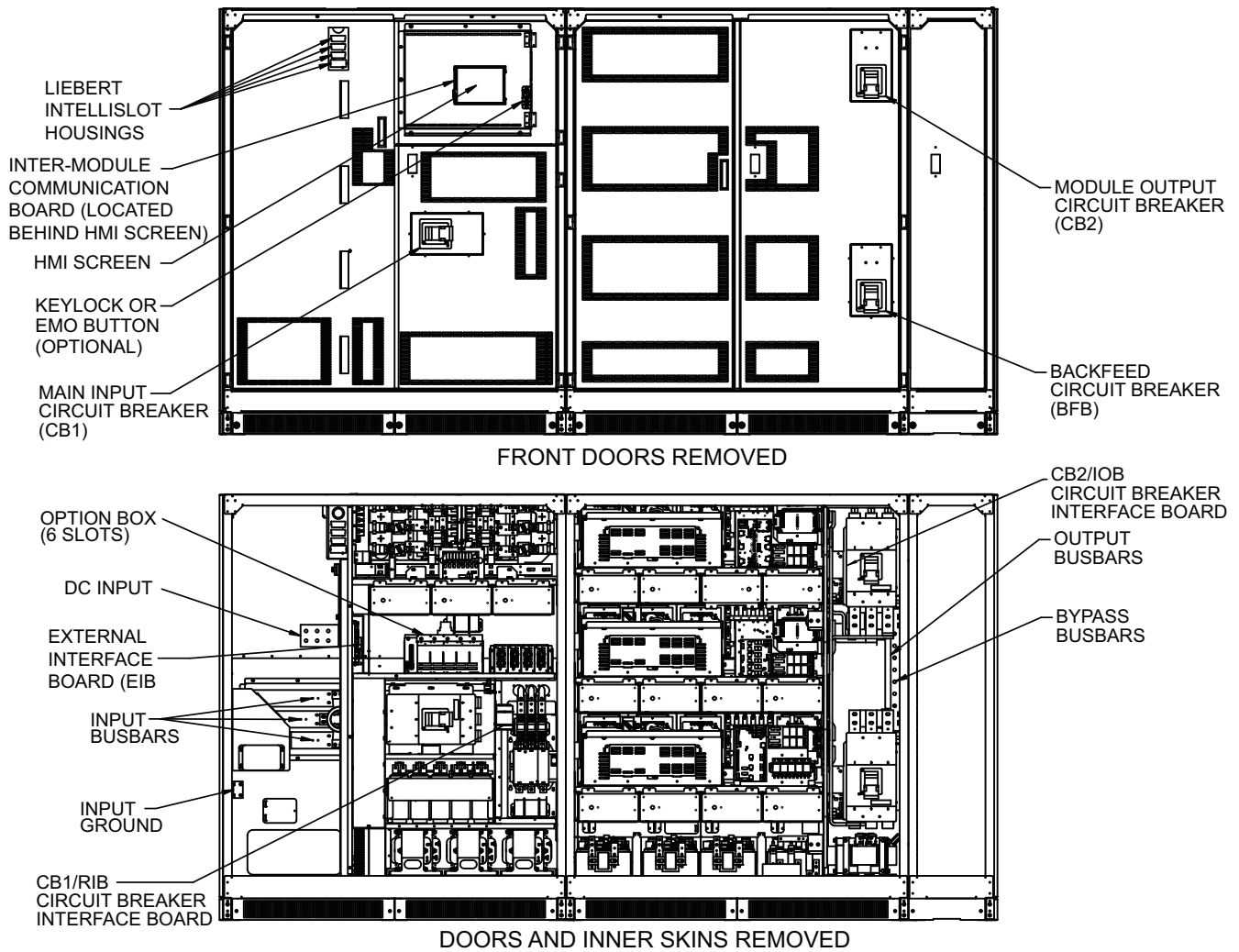
Figure 22 Main components, 625/750kVA Liebert NXL UPS, SMS and 1+N multi-module unit with static bypass
