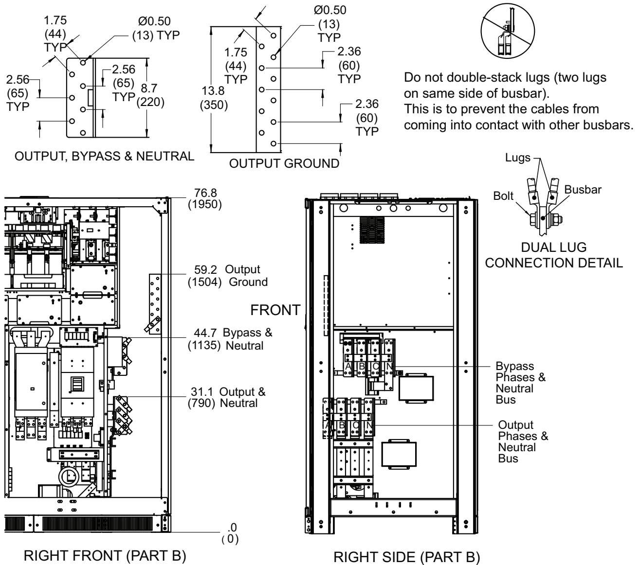
Figure 17 Output terminal details, Liebert NXL 500kVA UPS, SMS and 1+N multi-module unit with static bypass
