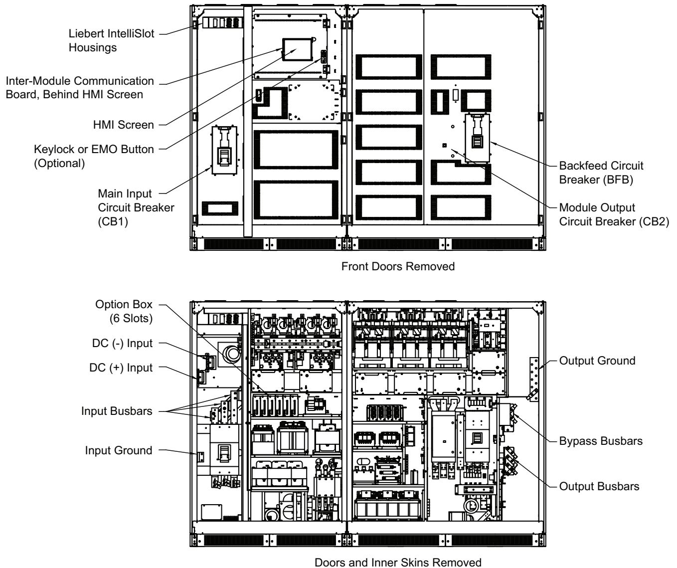
Figure 14 Main components, 500kVA Liebert NXL SMS and 1+N multi-module unit with static bypass
