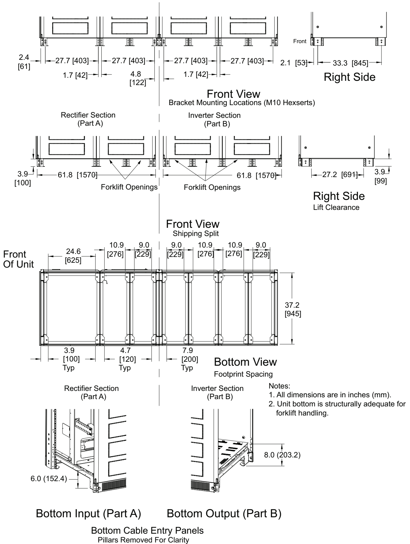
Figure 25 Base detail drawing, 625/750kVA Liebert NXL, N+1 multi-module unit without static bypass
