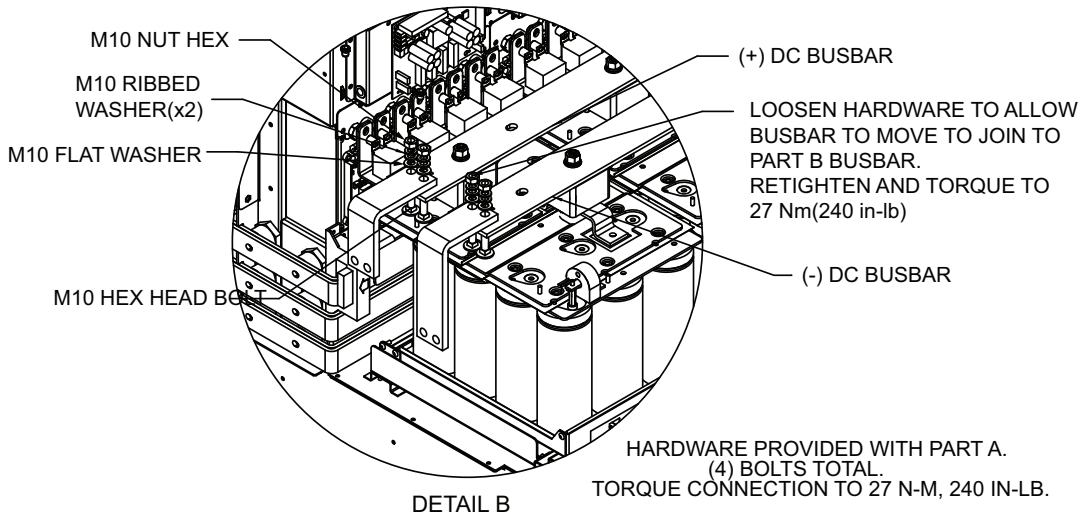
DC POWER CONNECTION BETWEEN PART B AND A.
