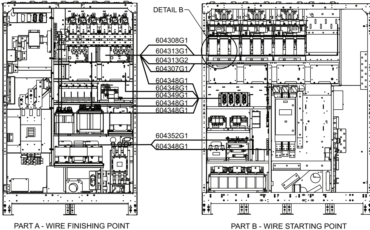
Figure 20 Field connections, shipping split 500kVA Liebert NXL, multi-module or SMS with static bypass, Page 2
