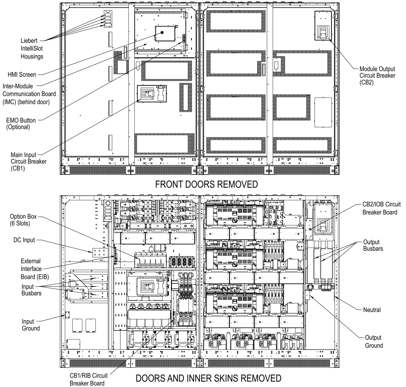
Figure 21 Main components, 625/750kVA Liebert NXL, N+1 multi-module unit without static bypass
