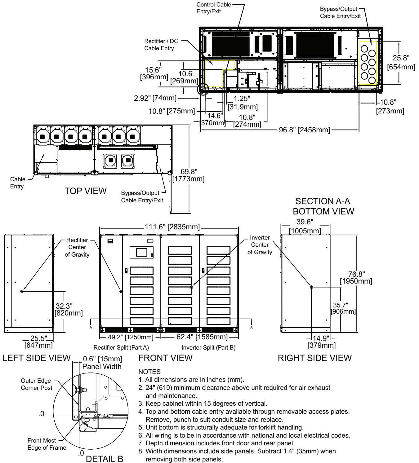
Figure 15 Outline drawing, Liebert NXL 500kVA UPS SMS and 1+N multi-module unit with static bypass
