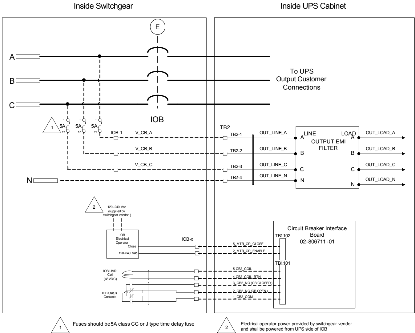
Figure 8 Remote Output Breaker diagram
