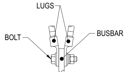
DUAL LUG CONNECTION DETAIL
