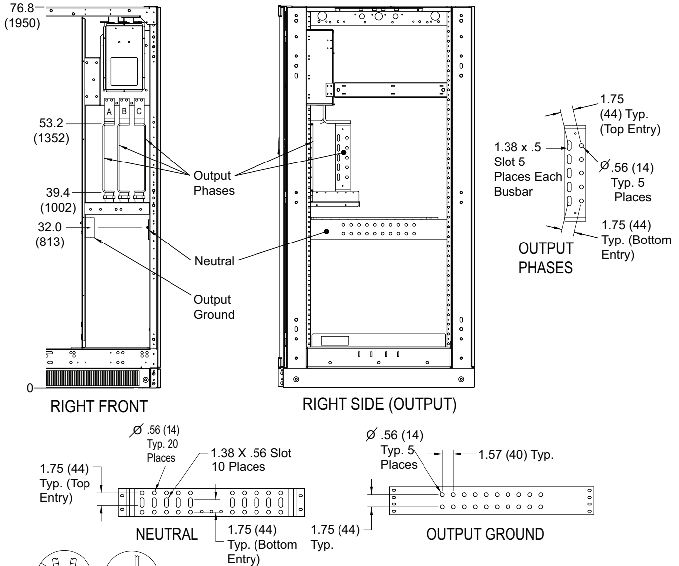
Figure 29 Output terminal detail, 625/750kVA Liebert NXL, N+1 multi-module unit without static bypass (continued)
