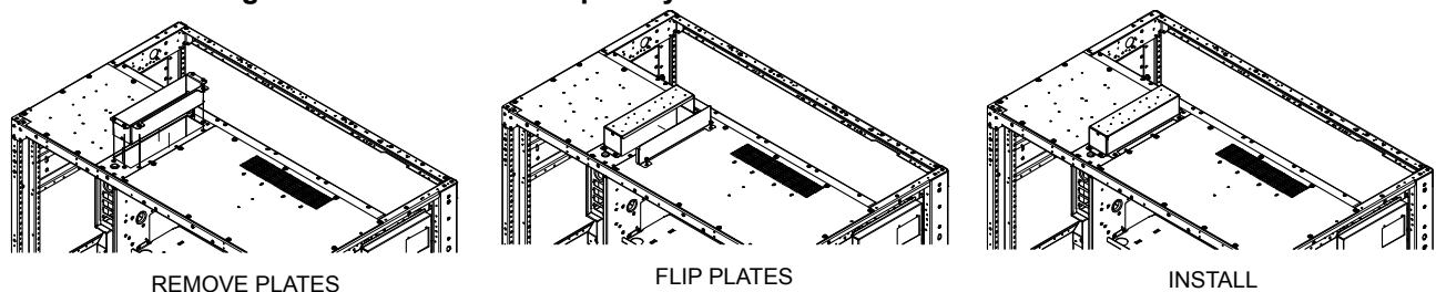
Figure 4 Low-voltage cable installation—top entry
