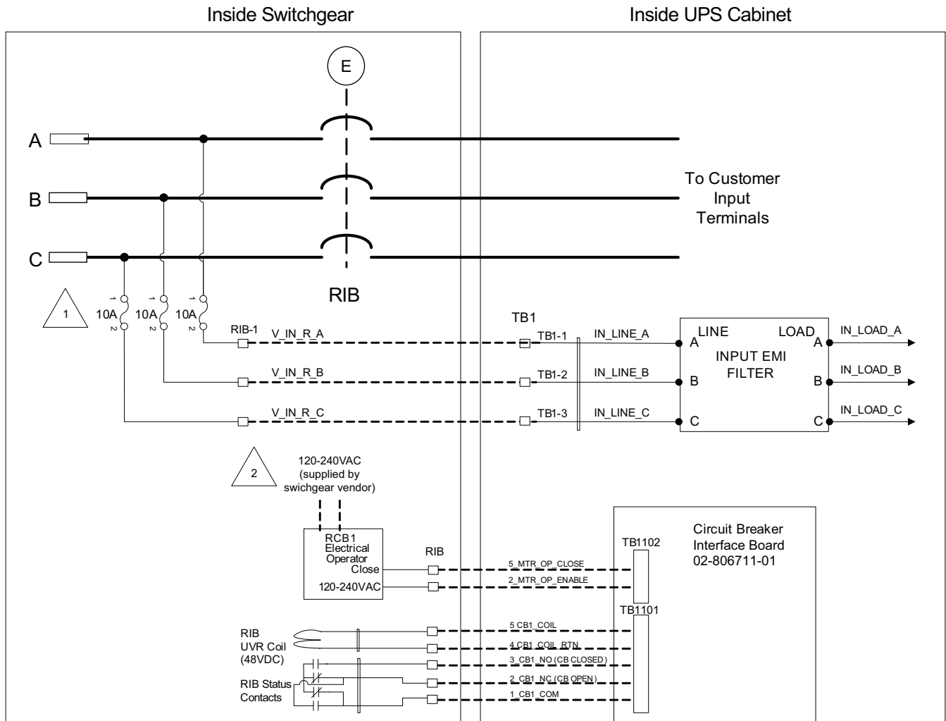
Figure 7 Remote Input Breaker diagram
