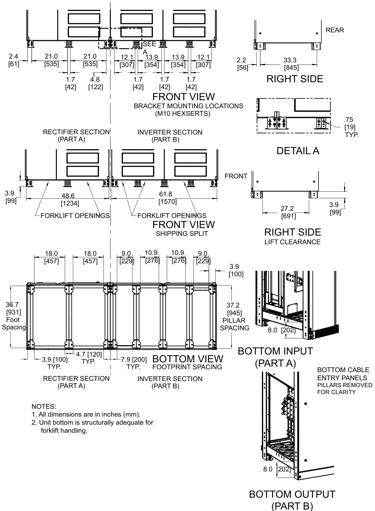
Figure 18 Base drawing, Liebert NXL 500kVA UPS, SMS and 1+N multi-module unit with static bypass
