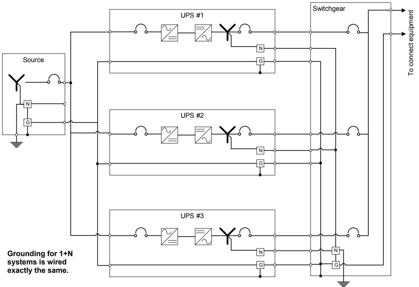
Figure 12 Grounding diagram, three-wire multi-module system
