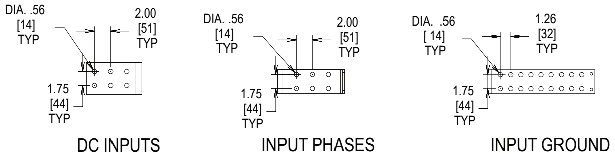
Figure 28 Input terminal detail, 625/750kVA Liebert NXL, SMS and 1+N multi-module unit with static bypass
