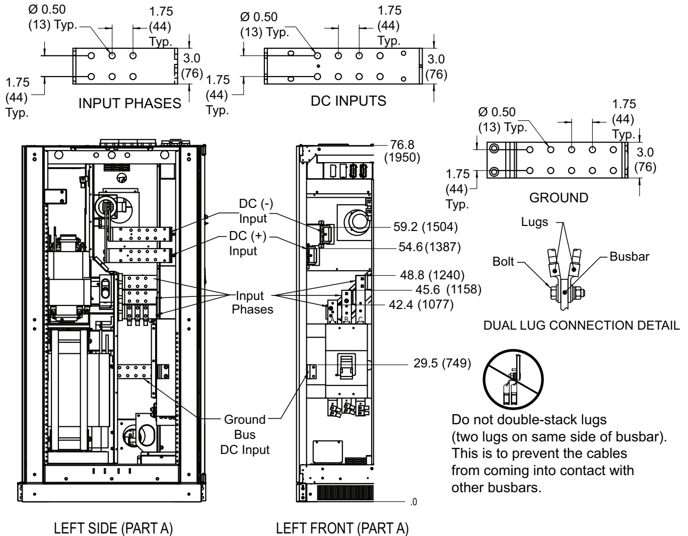
Figure 16 Input terminal details, Liebert NXL 500kVA UPS, SMS and 1+N multi-module unit with static bypass
