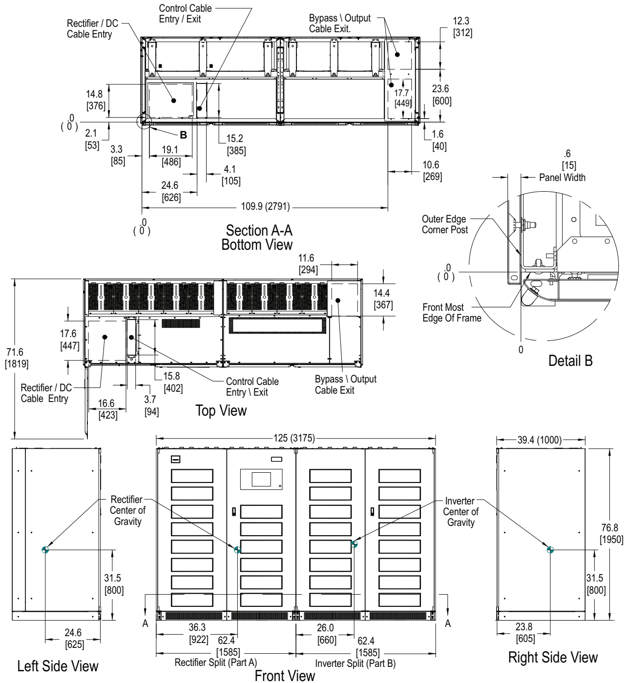
Figure 23 Outline drawing, 625/750kVA Liebert NXL, N+1 multi-module unit without static bypass
