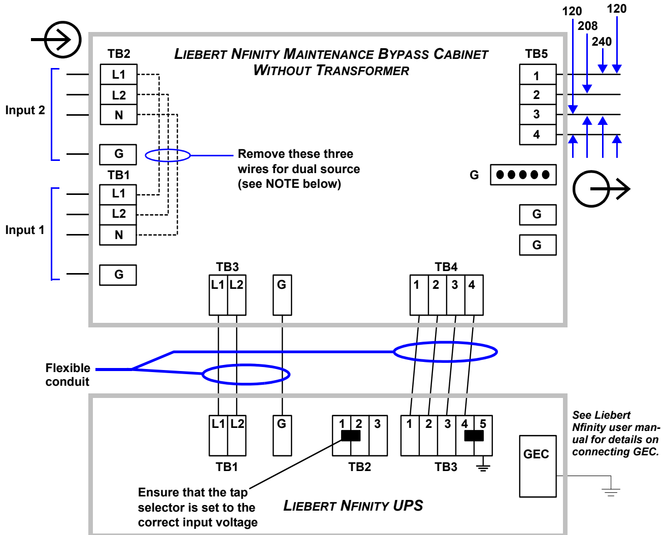
Figure 12 Connecting Liebert Nfinity to a Liebert Maintenance Bypass Cabinet without transformer
