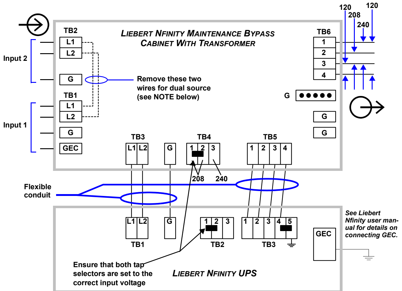
Figure 11 Connecting Liebert Nfinity to Liebert Nfinity Maintenance Bypass with transformer
