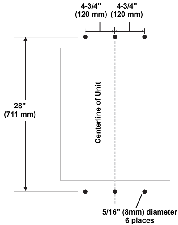
Top View of Liebert Nfinity Maintenance Bypass Cabinet
