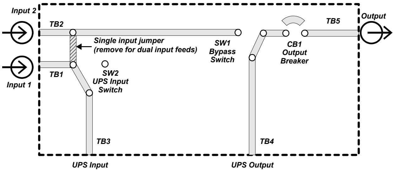
Figure 8 Liebert Nfinity Maintenance Bypass Cabinet without transformer
