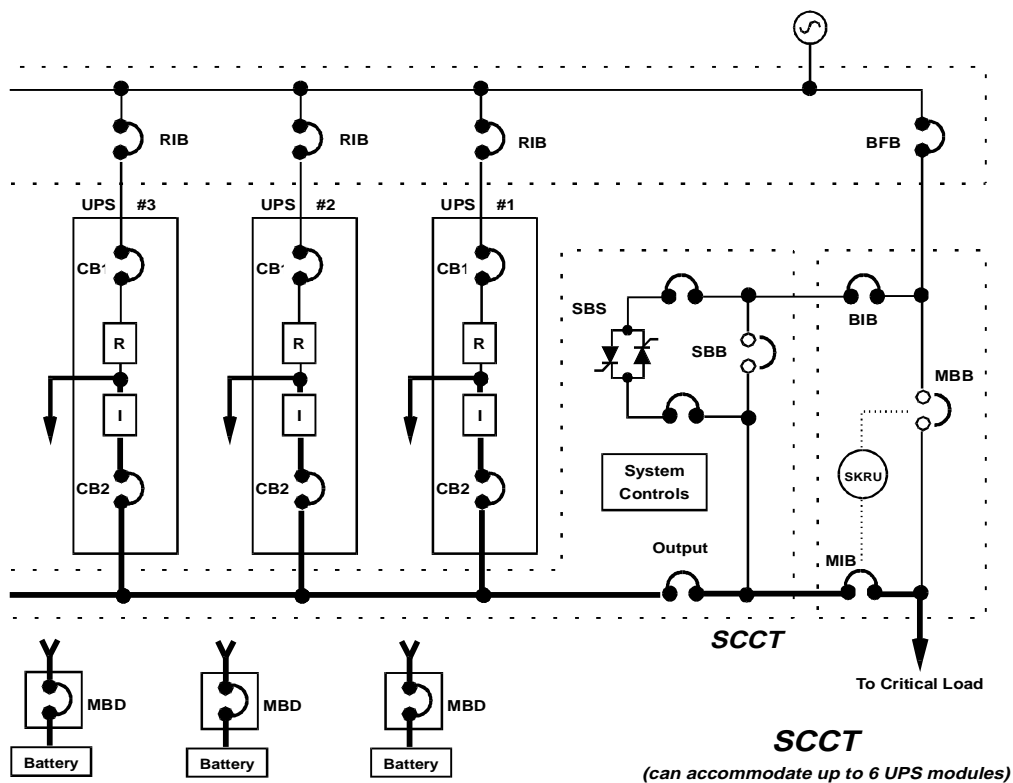
Figure 51 Input Power Fail (Load on Battery)
