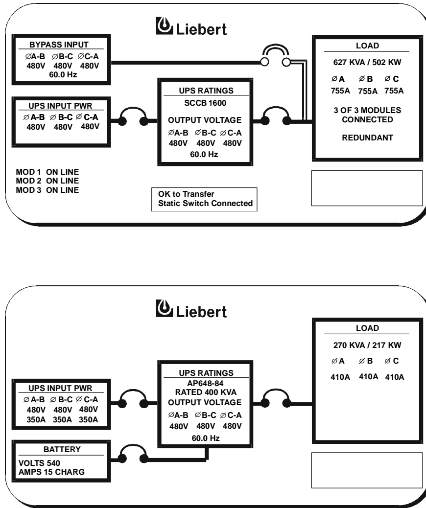
Figure 16 Monitor/Mimic Display Screen Examples: Normal Power Flow, SCC (above) and Module
