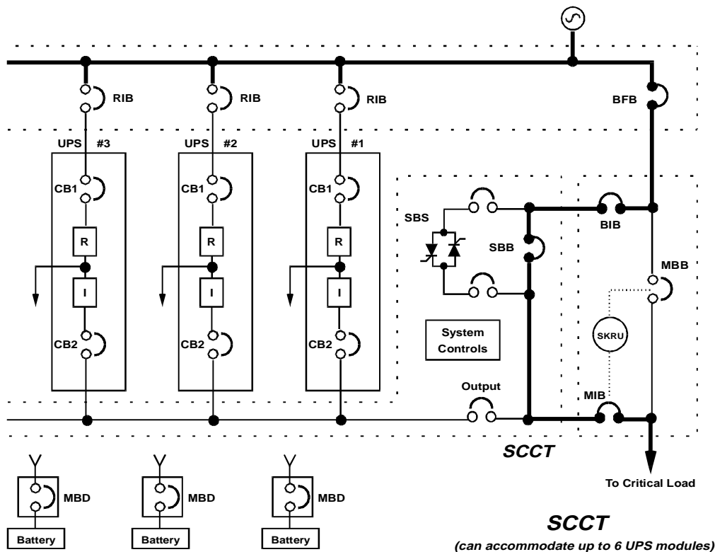
Figure 47 Load on Bypass (UPS Not Available)
