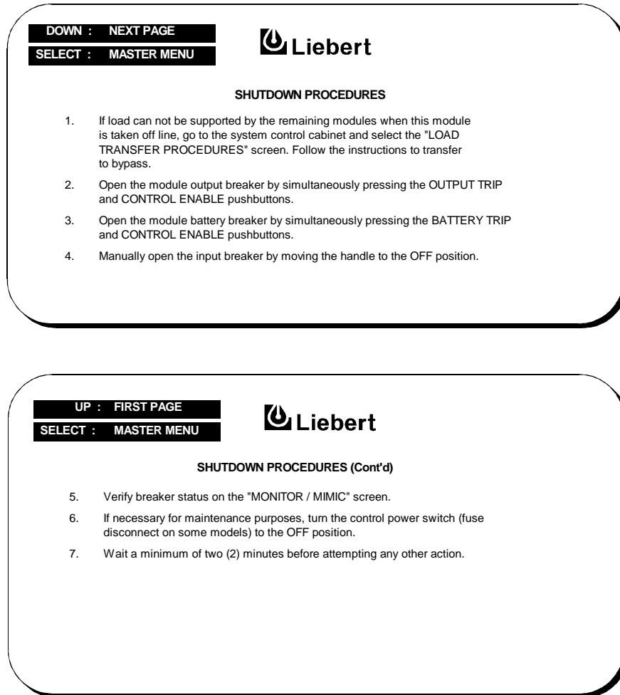
Figure 40 Module Shutdown Procedures Screen
