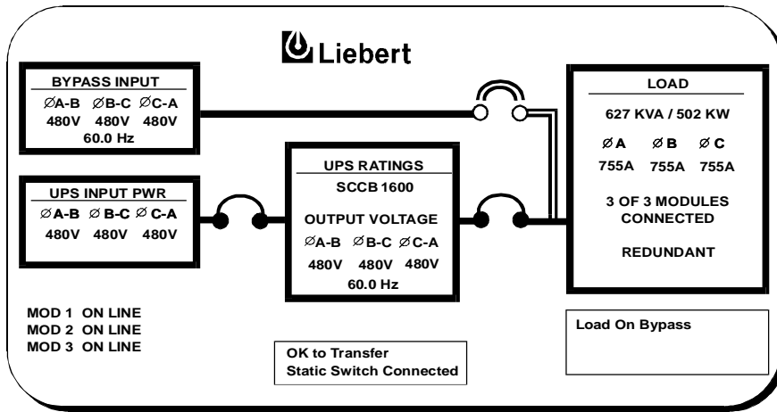
Figure 18 Monitor/Mimic Display Screen Examples: Load on Bypass, UPS Modules On and Charging Battery, SCC (above) and Module
